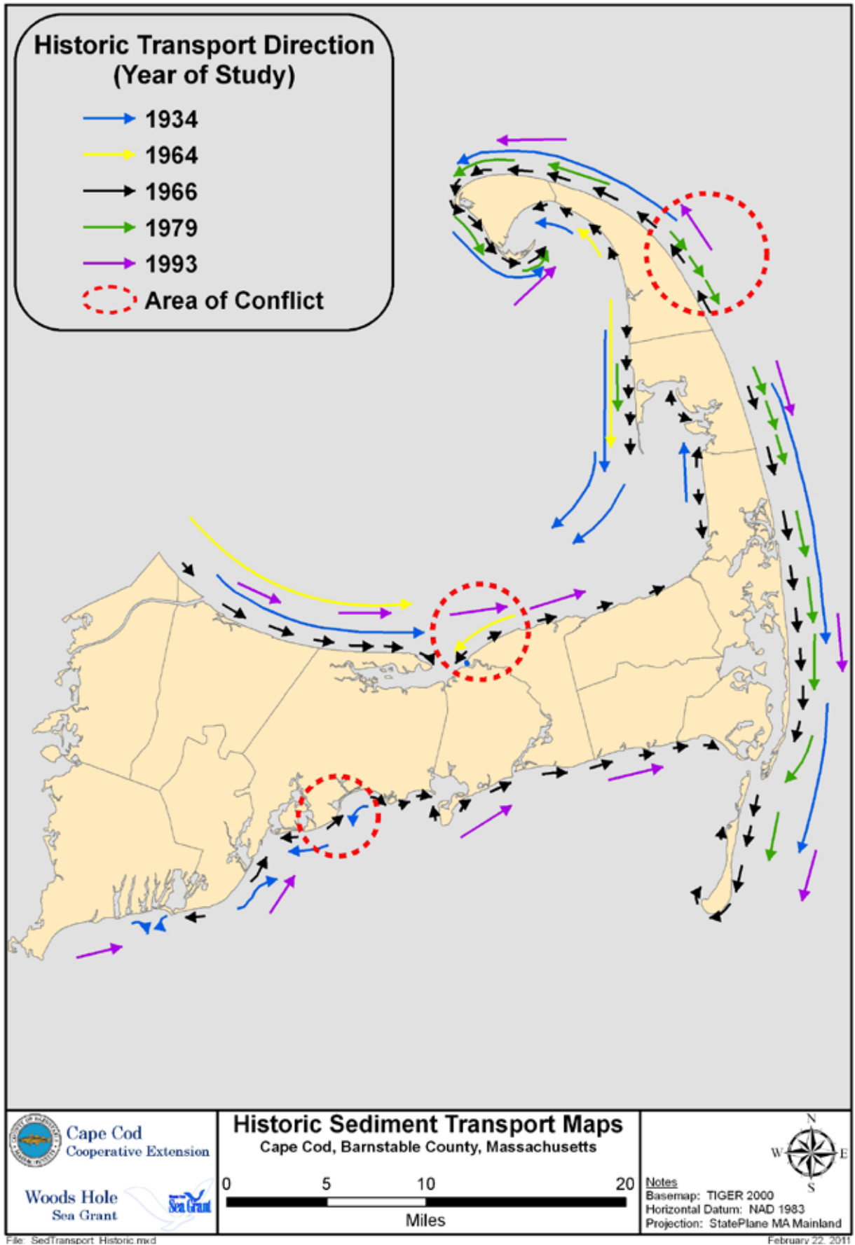
Figure 4. Composite historic transport map showing transport of sediment throughout the Cape Cod region. Each of the component maps was georeferenced and the arrows converted to vectors. The arrow length and position is depicted similarly to the original study map, except in cases where overlaps made the arrows illegible. Each study is color-coded according to the legend (Woodworth and Wigglesworth, 1934. Giese, 1964, Strahler, 1966. Fisher, 1979. FitzGerald, 1993.) Giese (1964 data) analysis based in part on previous studies (U.S. Congress, 1959 & 1960).
